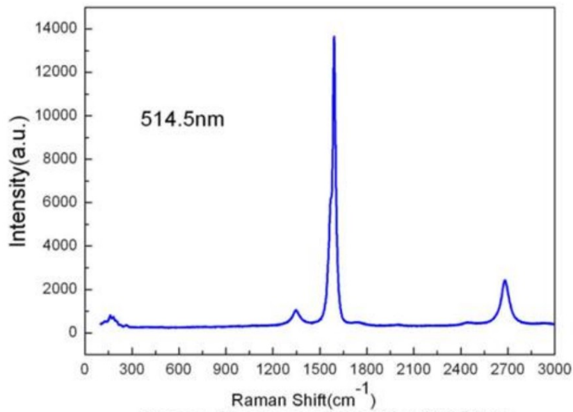
Raman Spectrum of Folating
